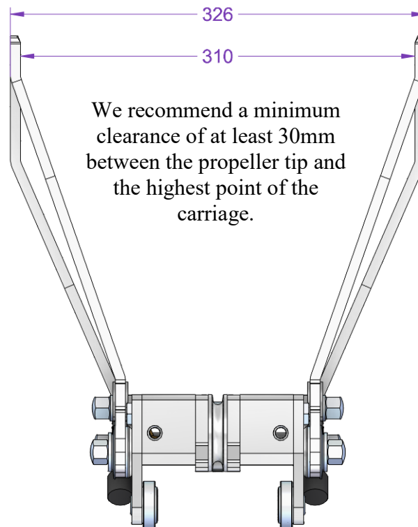
Figure 10-4 Standard carriage II dimensions.
