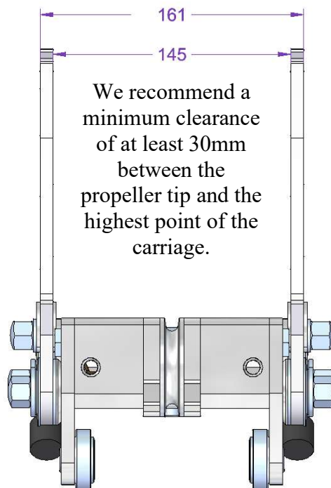
Figure 10-3 Standard carriage I dimensions
