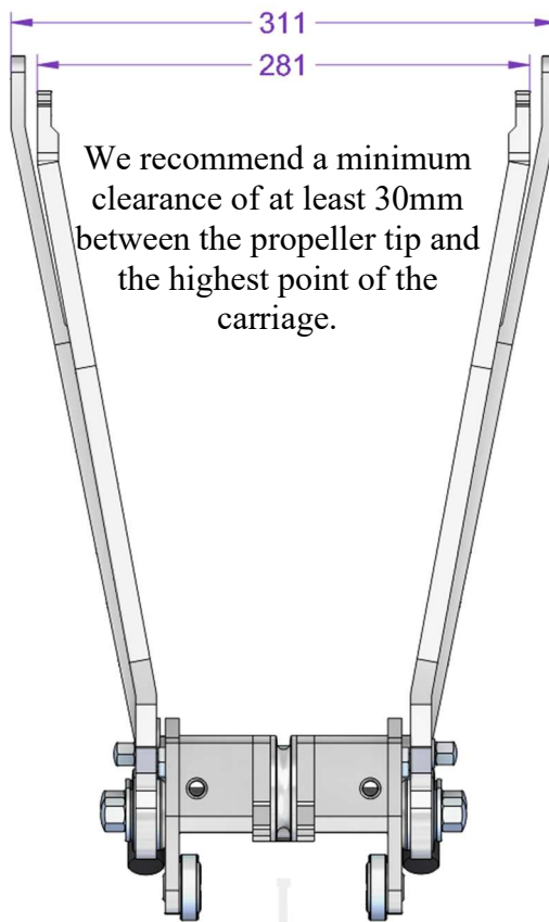
Figure 10-4 Standard carriage II dimensions.
