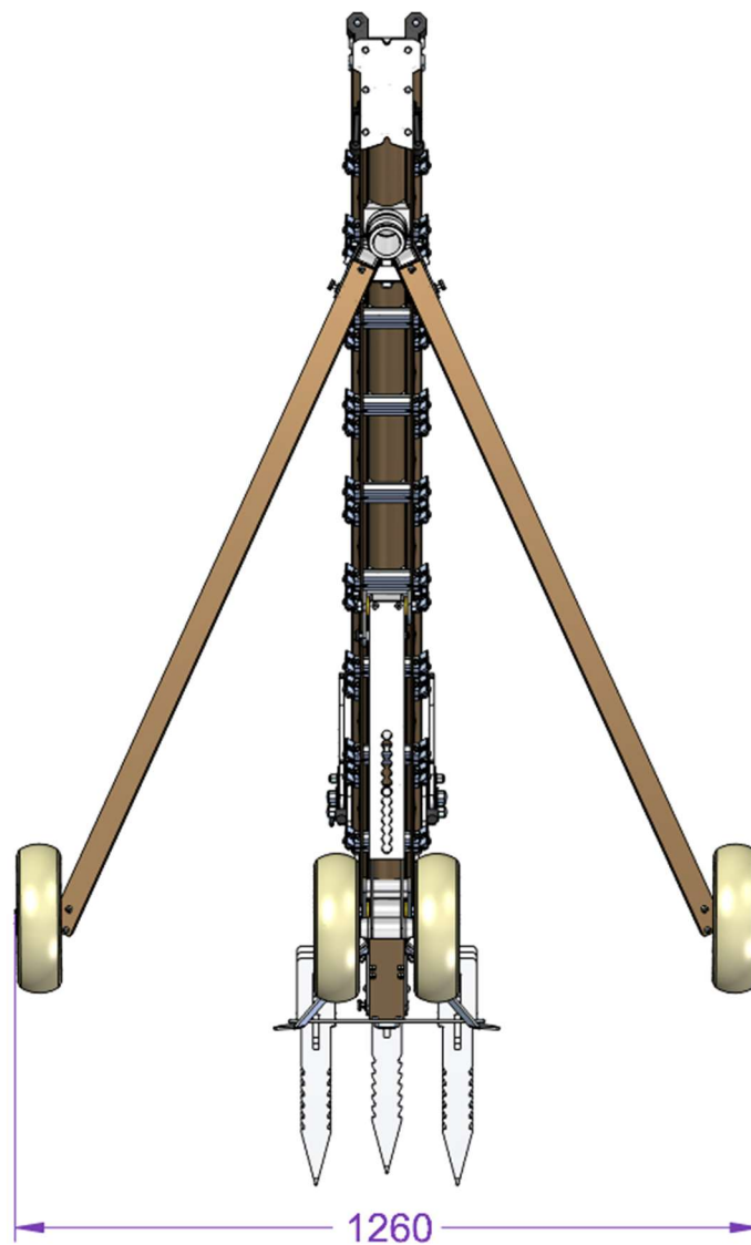
Figure 10-1 Overall dimensions when the PL-80 is assembled.
